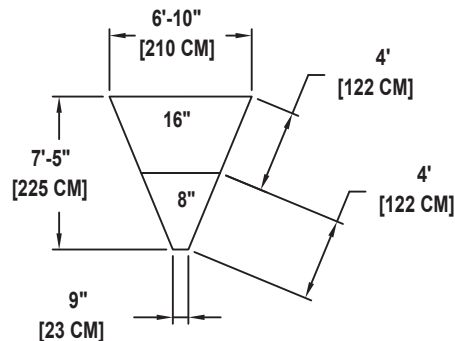
RISER SET 1135 SEATING CAPACITY 2
