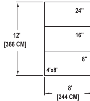
RISER SET 015 SEATING CAPACITY 9 (12 WITH A ROW ON THE FLOOR)
