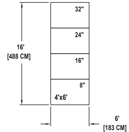
RISER SET 1225 SEATING CAPACITY 8 (10 WITH A ROW ON THE FLOOR)
