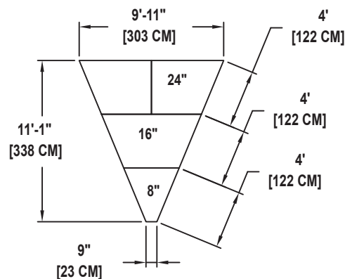
RISER SET 035 SEATING CAPACITY 4
