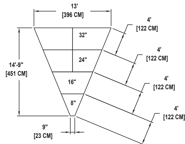
RISER SET 1235 SEATING CAPACITY 7
